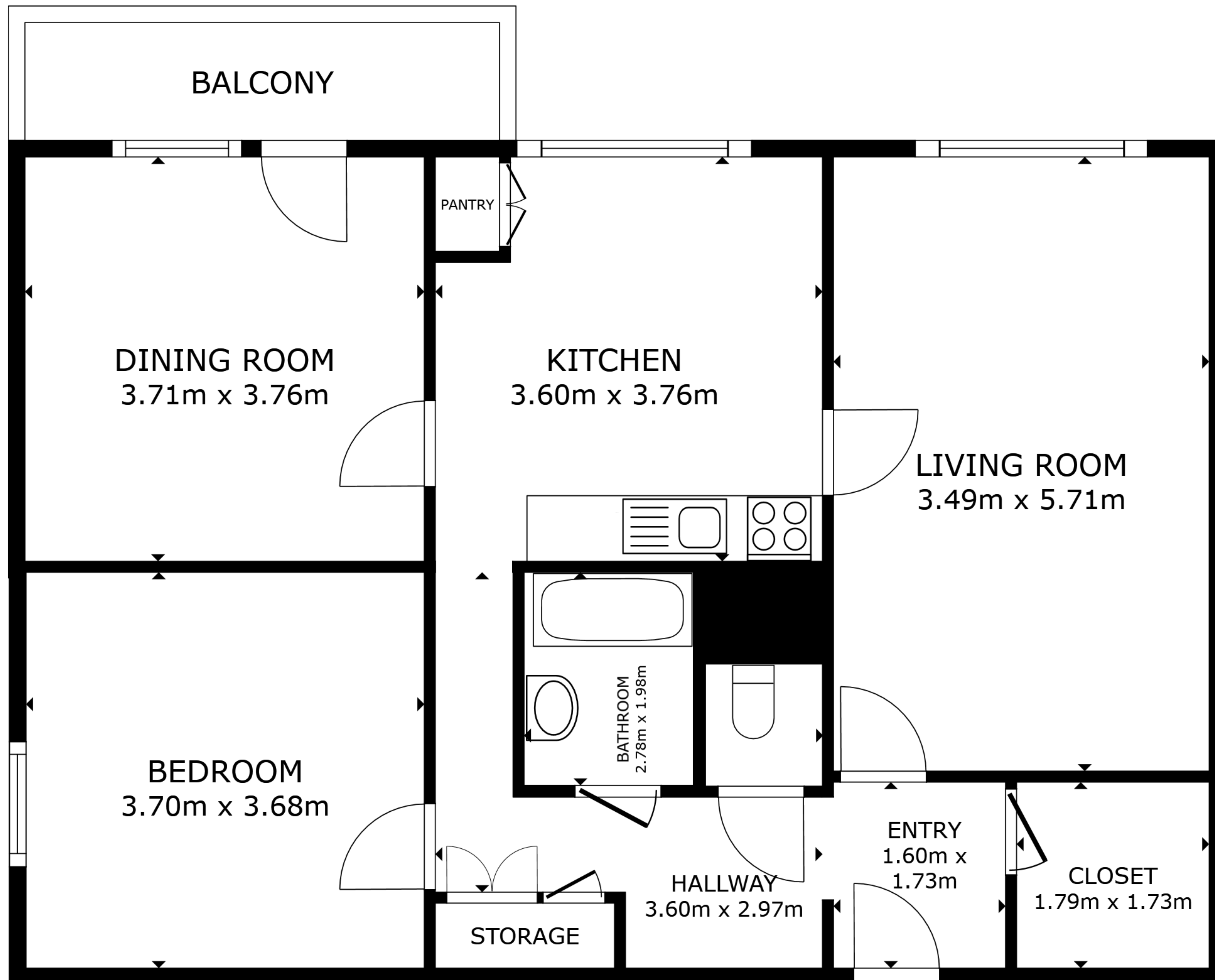
FLOOR PLAN
